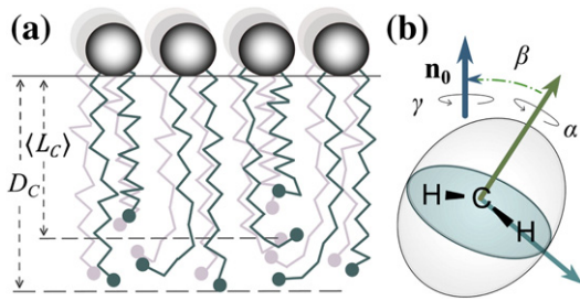
Fig. 3. Volumetric bilayer thickness is related to acyl chain projection onto the lamellar normal together with packing of the lipid segments. (a) Schematic representation of methylene chain travel from the lipid head group–water interface. The polar head groups are designated by large shaded spheres and the methyl groups at the acyl ends by the filled spheres. Note that the acyl chains are more disordered at the middle of the bilayer. The mean acyl length \langle L_C \rangle is less than the volumetric half-thickness D_C of the bilayer. (b) Orientations of \text{CH}_2 segments and their projection onto the bilayer normal \mathbf{n}_0 are related to the average thickness of the membrane. In ^2\text{H} NMR spectroscopy hydrogen (H) is substituted by deuterium. The spatial orientation of an acyl segment is represented by three Euler angles \Omega \equiv (\alpha, \beta, \gamma) , where \beta \equiv \beta_{iM} for the i th segment. The average projection of the chains corresponds to the experimentally measured order parameters S_{CD}^{(i)} = \frac{1}{2} \langle 3 \cos^2 \beta_{PD}^{(i)}(t) - 1 \rangle in terms of the orientational distribution function.
