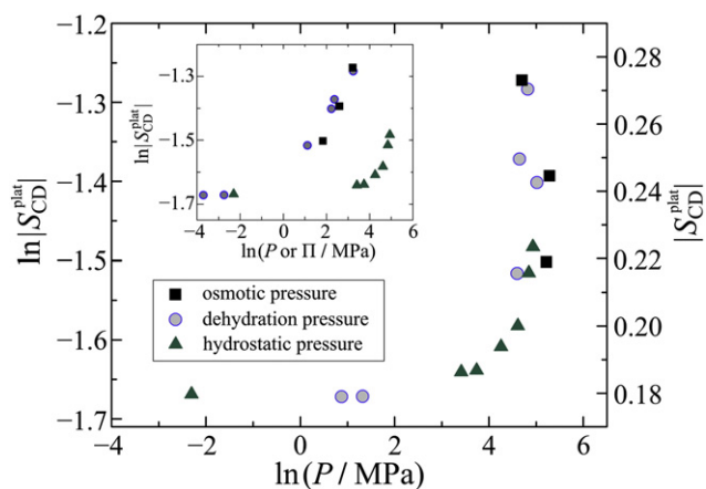
Fig. 6. Solid-state ^2\text{H} NMR spectroscopy enables comparison of various pressure-based measurements of lipid bilayer deformation for DMPC- d_{54} membranes in the liquid-crystalline state. The maximum ^2\text{H} NMR order parameter (plateau) |S_{\text{CD}}^{\text{plateau}}| values at 45^\circ\text{C} are plotted as a function of osmotic pressure (■) or dehydration [pressure] (●); and versus hydrostatic pressure (▲) by using the ^2\text{H} NMR order parameters as a secondary osmometer (see Refs. [3] and [26] for details). Inset: Comparison of order parameters plotted against external pressure applied in three different ways (dehydration, osmotic, hydrostatic). Note that ^2\text{H} NMR spectroscopy allows us to collapse the various pressure-based measurements to a single universal curve. Data are from Ref. [3].
