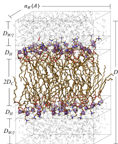
Fig. 2. Lipid bilayer showing schematic depiction of unit cell and structural measures obtained from solid-state ^2\text{H} NMR spectroscopy and small-angle X-ray scattering. Lamellar structure of the phospholipid membrane is shown with the pertinent structural quantities. The lamellar repeat spacing D = D_W + D_B is the sum of the interlamellar water distance D_W = 2D_{W/2} and the bilayer thickness D_B = 2(D_H + D_C) . Here D_C is the hydrocarbon thickness per bilayer leaflet and D_H is the head group layer thickness. Bilayer dimensions involve the average cross-sectional area per lipid \langle A \rangle , which together with the number of lipids ( N_L ) give the overall surface area of the membrane. Changes in equilibrium structural quantities due to bilayer stress give a membrane-based view of the forces that underlie lipid interactions within the bilayer.
