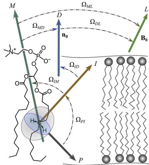
Fig. 4. Illustration of how the orientational distribution function describes average membrane structural properties by travel of the lipid segments. Hydrogen (H) is substituted by deuterium in solid-state ^2\text{H} NMR spectroscopy. The frame of the \text{C}-^2\text{H} bond is the principal axis system ( P ) for evaluating the segmental order parameter. The main external magnetic field \mathbf{B}_0 corresponds to the laboratory frame ( L ). Designations for the Euler angles \Omega \equiv (\alpha, \beta, \gamma) are: P , principal axis system for ^2\text{H} nucleus ( z -axis parallel to \text{C}-^2\text{H} bond); I , intermediate frame for methylene group motion ( z -axis perpendicular to \text{H}-\text{C}-\text{H} plane); M , molecular coordinate system; D , director frame ( z -axis is bilayer normal); and L , laboratory system ( z -axis along main external magnetic field \mathbf{B}_0 ). The closure property from group theory allows the overall rotation of the \text{C}-^2\text{H} bond to the laboratory frame to be expanded or collapsed in terms of various coordinate frames depending on the motional model.
