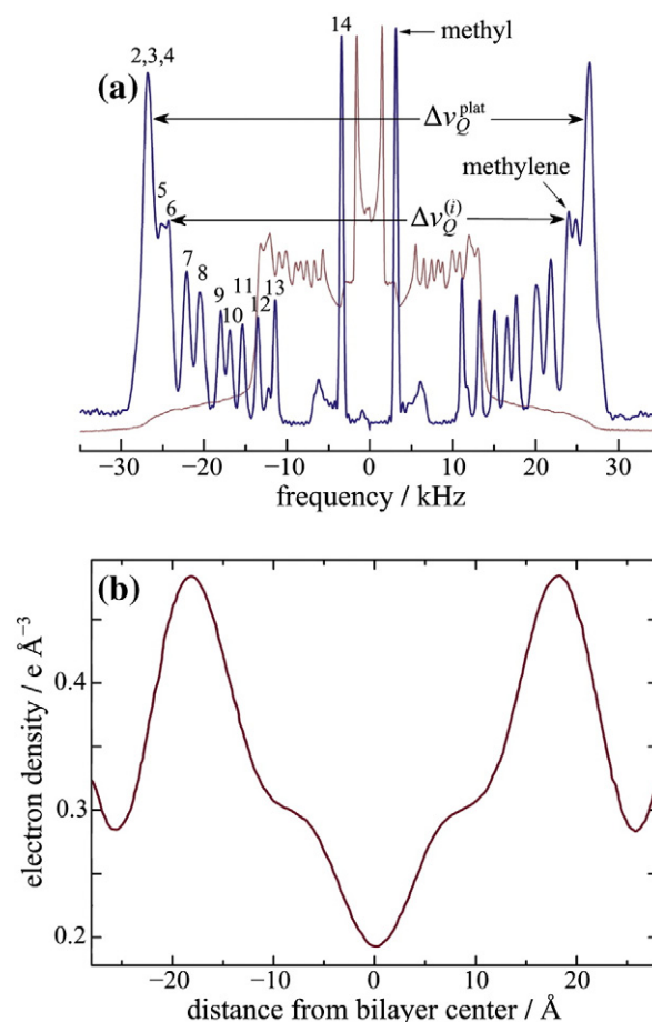
Fig. 1. Comparison of experimental methods used to study lipid membranes. (a) Solid-state ^2\text{H} NMR spectrum for multilamellar fully hydrated DMPC- d_{54} (with perdeuterated acyl groups) in the liquid-crystalline state at 30 °C recorded at 46.07 MHz (7.01 Tesla). The continuous thin line is the experimental powder-type spectrum and the thick line is the numerically deconvoluted (de-Paked spectrum). Numbers in the figure indicate the acyl chain carbon for each peak in the spectrum. Residual quadrupolar couplings (RQCs) are designated by \Delta\nu_Q^{(i)} and yield the absolute order parameters |S_{CH}^{(i)}| of the C– ^2\text{H} bonds directly, where i = 2 \dots 14 is the acyl chain segment index. (b) Electron density profile (absolute) for fully hydrated DMPC lipid bilayer at 30 °C obtained from small-angle X-ray scattering studies (SAXS) [47]. Two maximum peaks correspond to the electron-rich phosphodiester head groups on either side of the bilayer center. Positional order from SAXS is complementary to orientational order from solid-state ^2\text{H} NMR spectroscopy data giving atomistic detail for the lipid bilayer.
